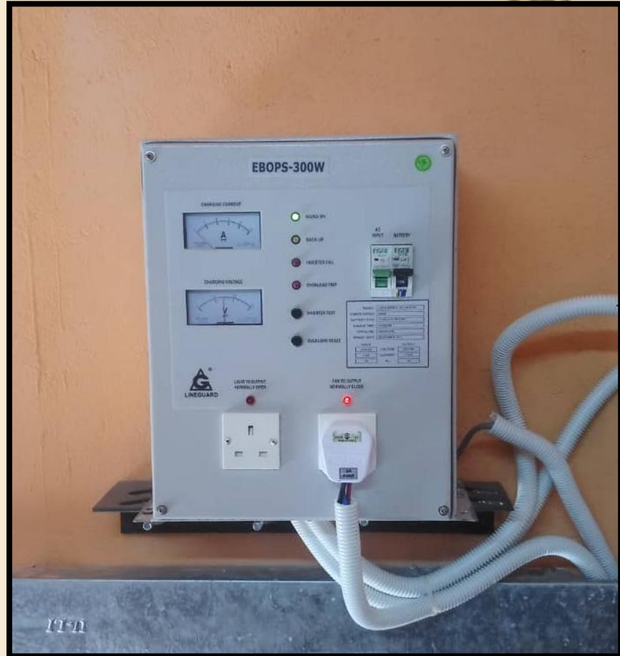
EMERGENCY BATTERY OPERATED POWER SUPPLY (EBOPS)
