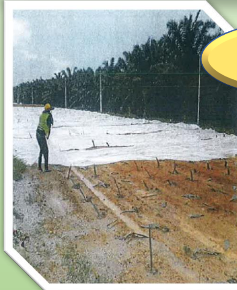
REMOVAL OF UNSUITABLE MATERIAL (USM)
