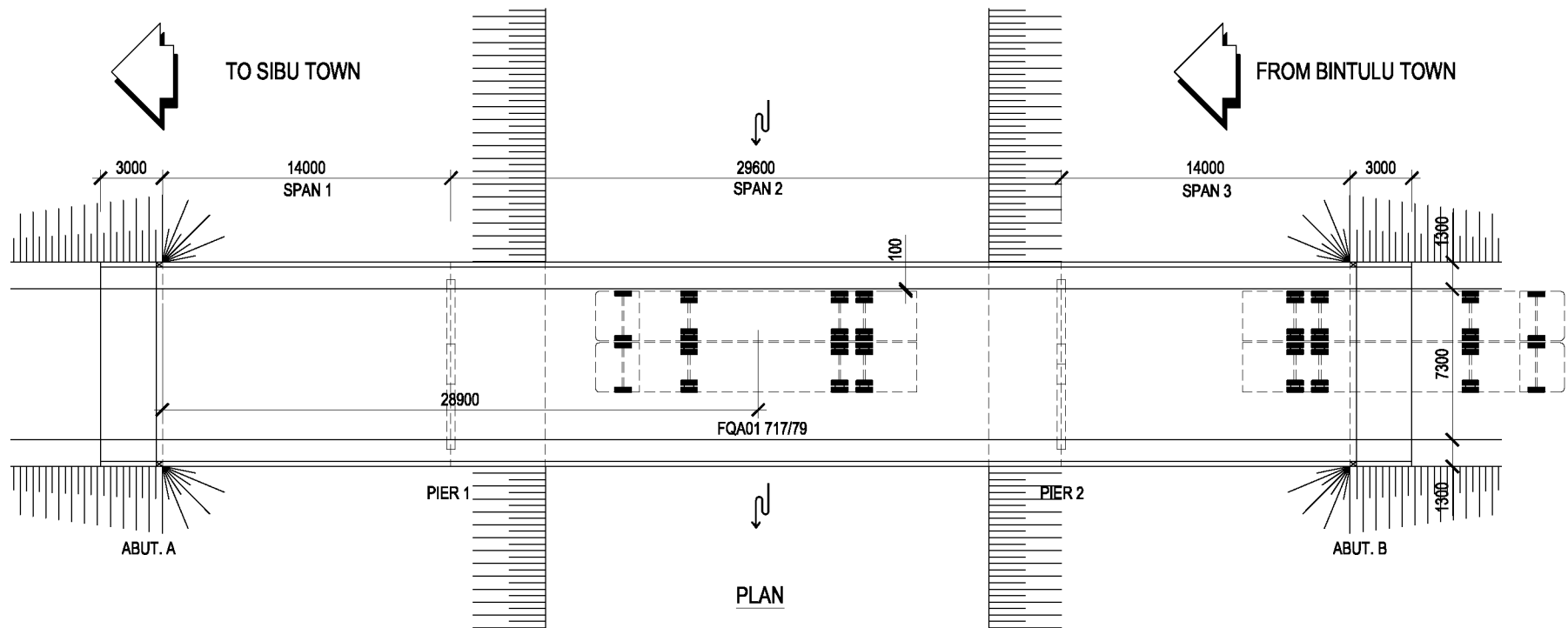
FIGURE 3 POSITION FOR HOGGING MOMENT
