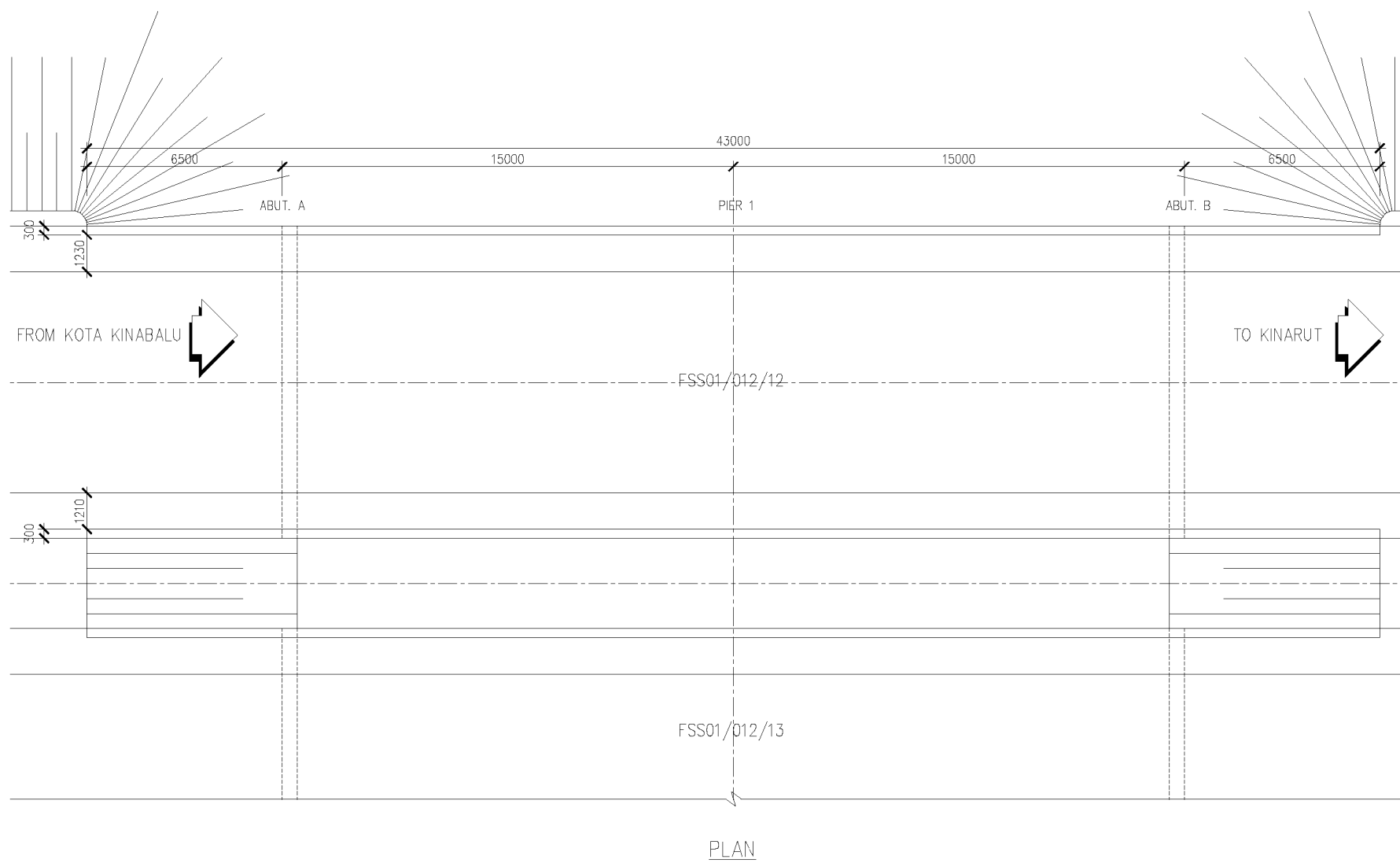
FIGURE 1 GENERAL ARRANGEMENT
