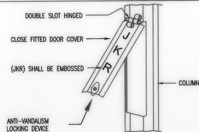
DETAIL 3: DOUBLE SLOT HINGED RIVETED TO COLUMN
