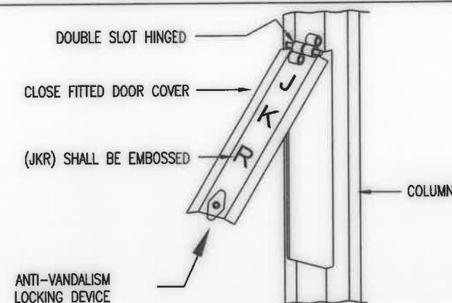
DETAIL 5: HINGED DOOR ISOMETRIC VIEW
