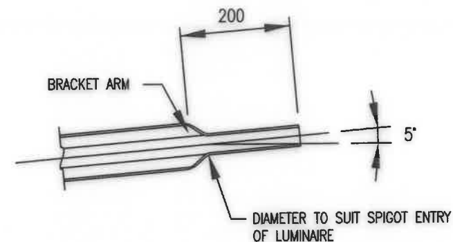
DETAIL 1: SPIGOT END OF BRACKET ARM
