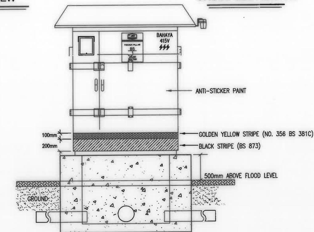
STANDARD PAINTING FOR JKR'S FEEDER PILLAR
