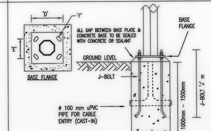
DETAIL 6: BASE FLANGED & CONCRETE FOUNDATION
