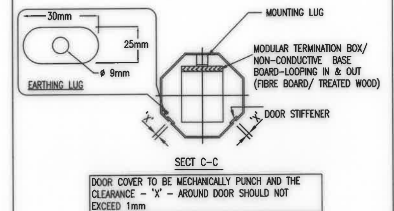
DETAIL 4: BASE BOARD FOR TERMINATION BOX
