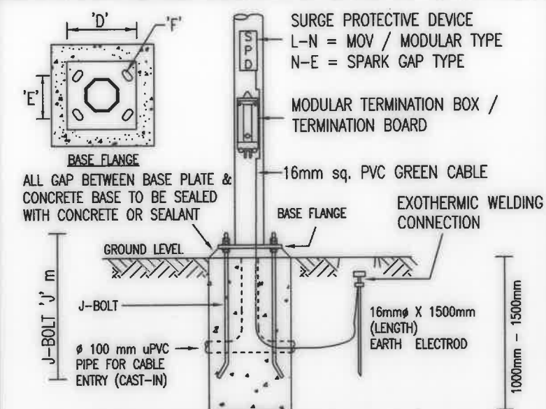
DETAIL 6: BASE FLANGED & CONCRETE FOUNDATION
