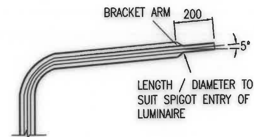
DETAIL 1: SPIGOT END OF BRACKET ARM
