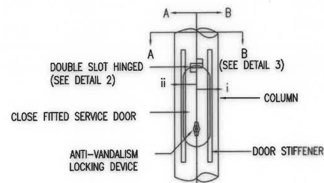
DETAIL 1: DOUBLE SLOT HINGED SERVICE DOOR
