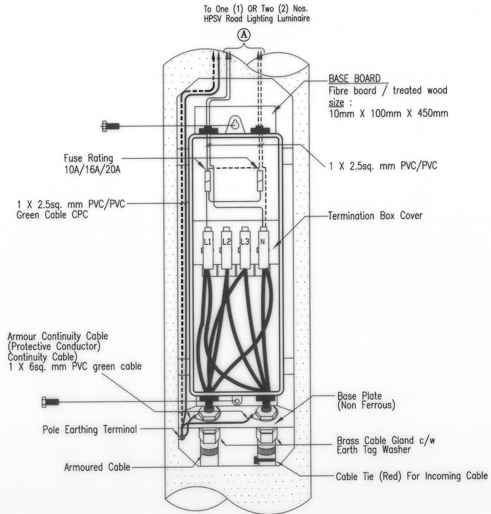
MODULAR TERMINATION BOX C/W LOOPING IN & OUT CABLE IN ROAD LIGHTING COLUMN
