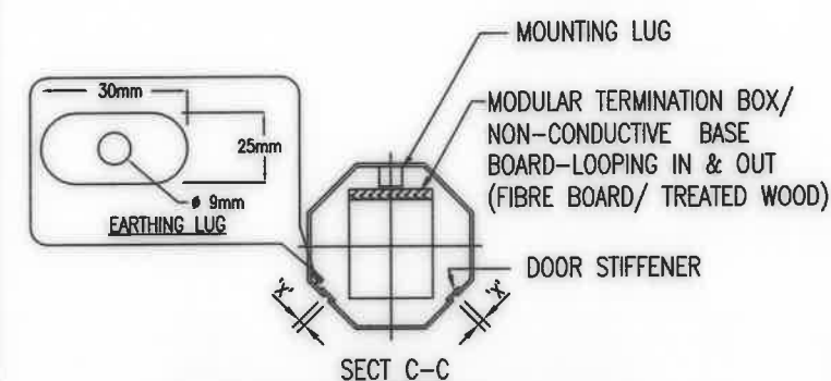
DETAIL 2: DOUBLE SLOT HINGED SERVICE DOOR
