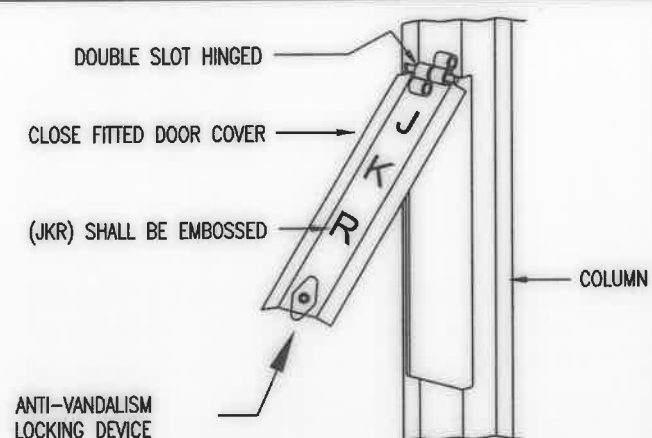
DETAIL 4: HINGED DOOR ISOMETRIC VIEW
