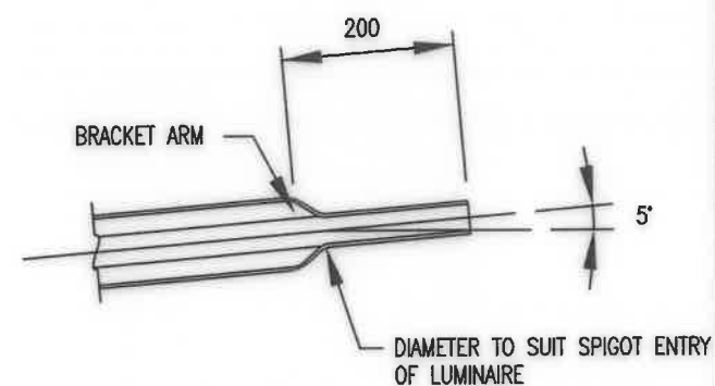
DETAIL 1: SPIGOT END OF BRACKET ARM
