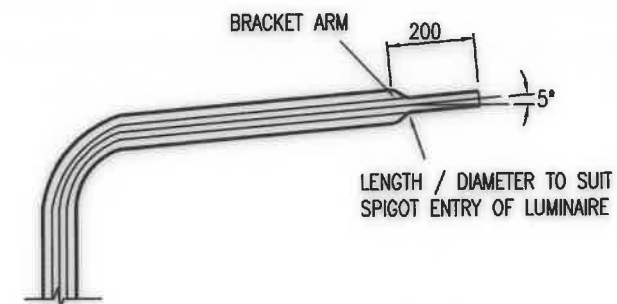
DETAIL 1: SPIGOT END OF BRACKET ARM
