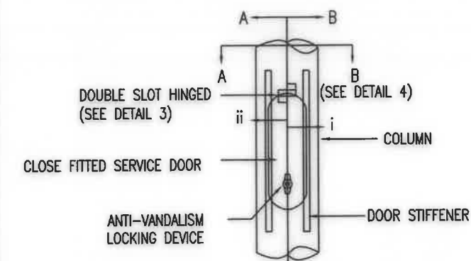
DETAIL 2: DOUBLE SLOT HINGED SERVICE DOOR
