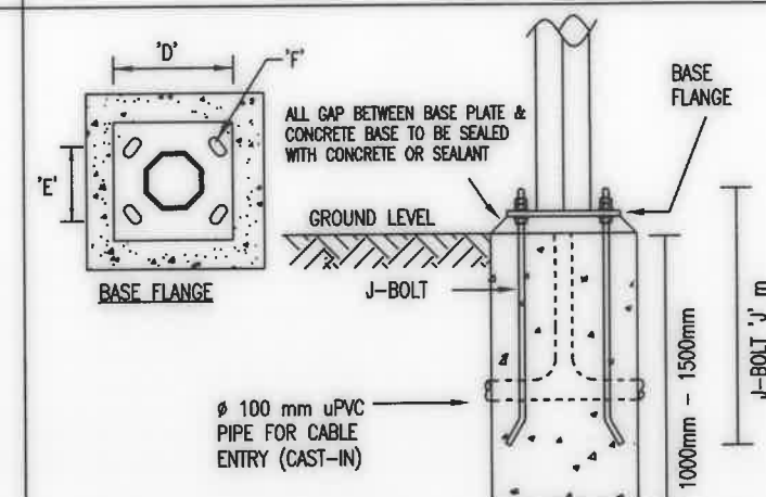
DETAIL 6: BASE FLANGED & CONCRETE FOUNDATION
