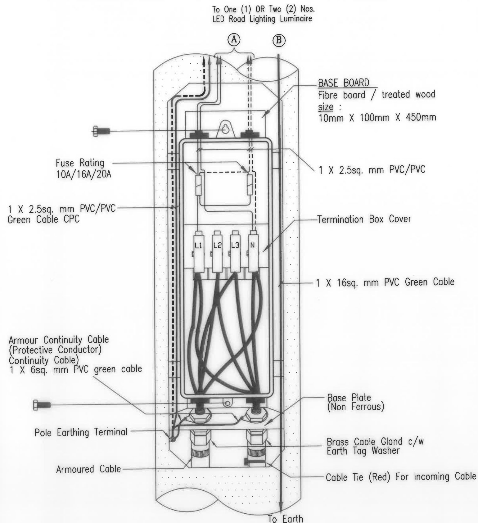
MODULAR TERMINATION BOX C/W LOOPING IN & OUT CABLE ROAD LIGHTING COLUMN
