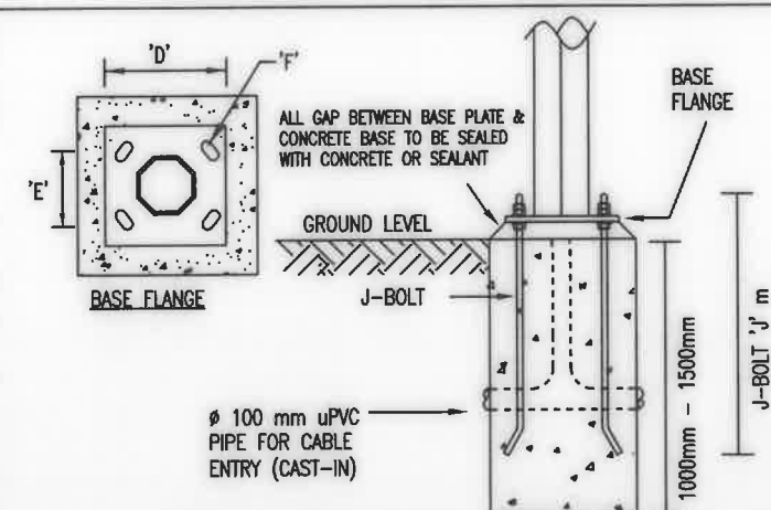
DETAIL 5: BASE FLANGED & CONCRETE FOUNDATION
