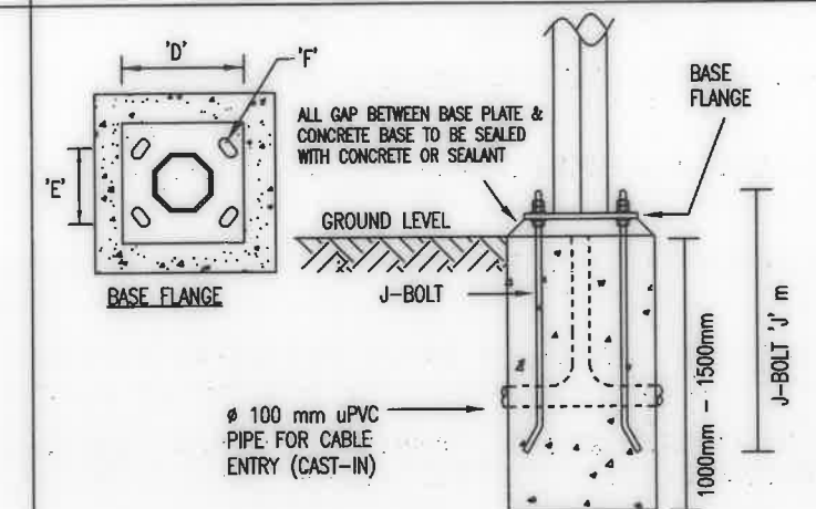
DETAIL 6: BASE FLANGED & CONCRETE FOUNDATION
