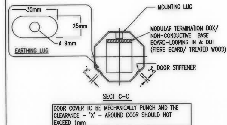
DETAIL 4: BASE BOARD FOR TERMINATION BOX
