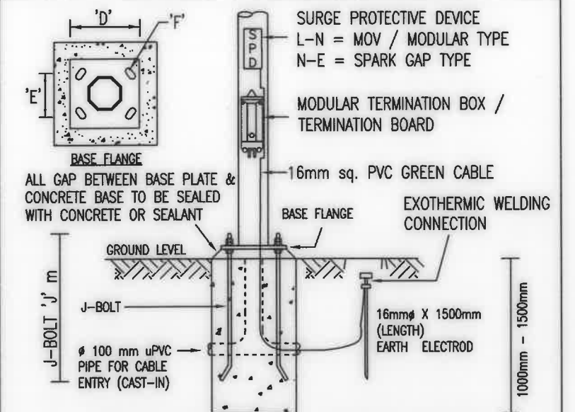
DETAIL 6: BASE FLANGED & CONCRETE FOUNDATION
