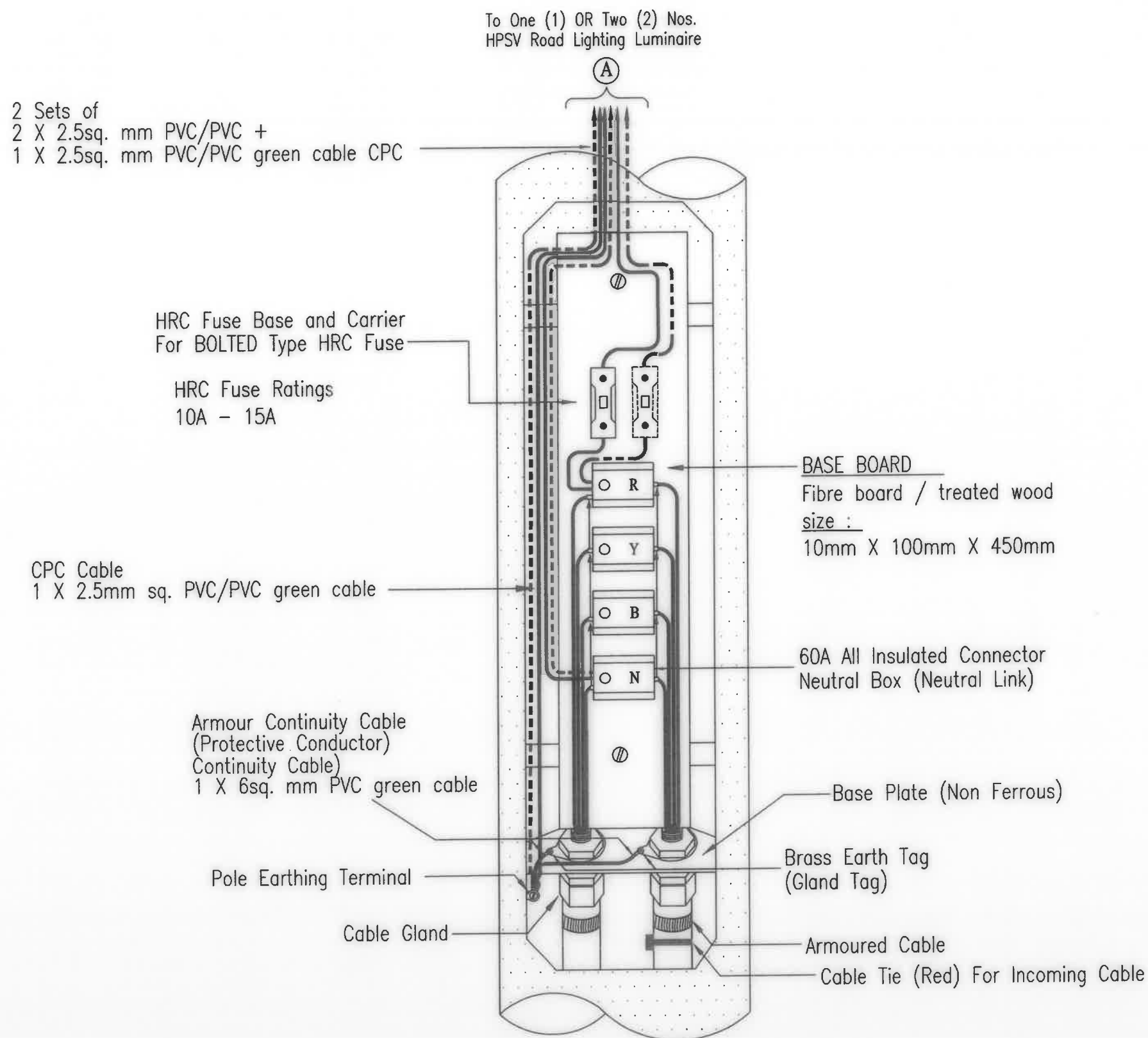
TERMINATION BOARD C/W LOOPING IN & OUT CABLE IN ROAD LIGHTING COLUMN
