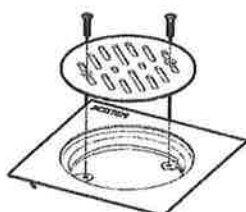
6R816SS-1 Center Round Grating Fastening by 2 nos. M5 X 20mm Steel Screws
