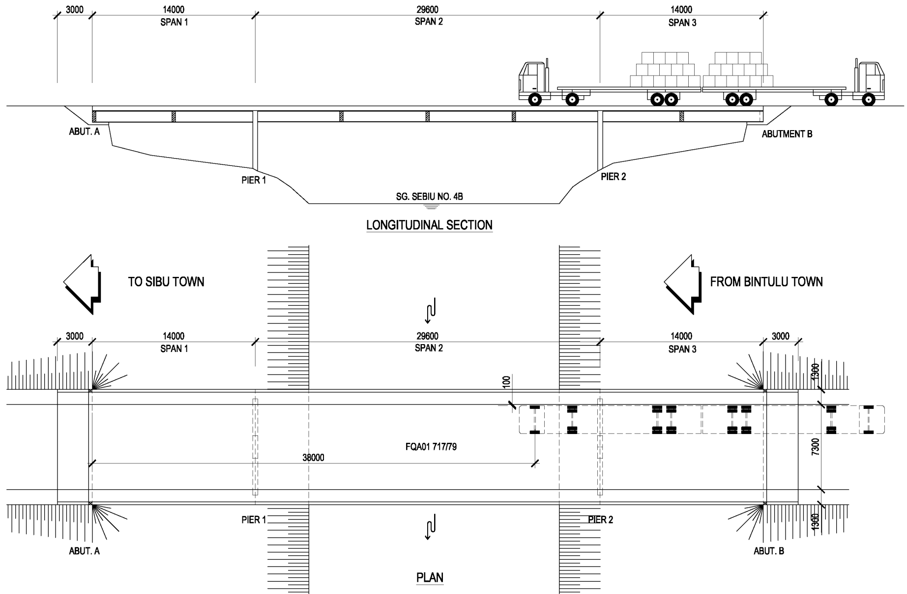
FIGURE 2 POSITION FOR SAGGING MOMENT AND SHEAR
