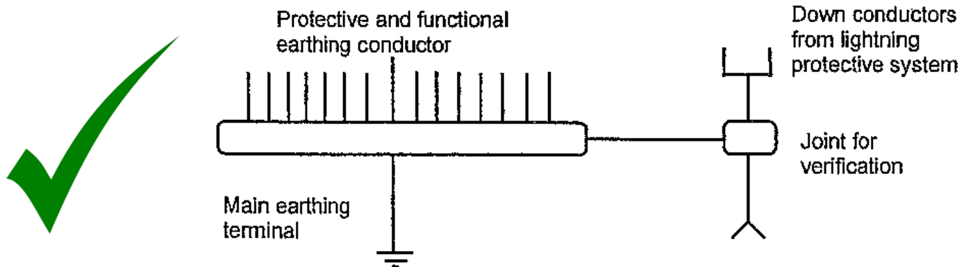
Interconnected earth electrodes
