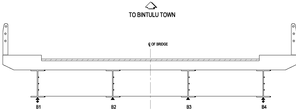
FIGURE 5: POSITION OF STRAIN GAUGES, LVDT AND PRECISE LEVEL IN BEAM AT MID SPAN
