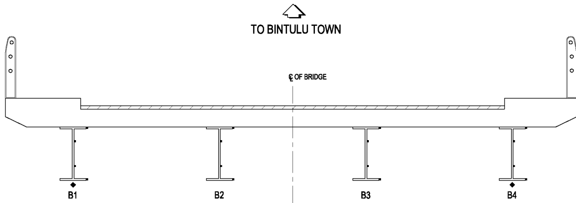
FIGURE 6: POSITION OF STRAIN GAUGES AND PRECISE LEVEL AT PIER 2
