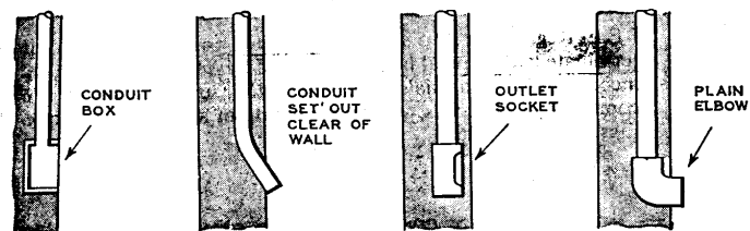
Fig. 5.26. I.E.E. Regulation B.69 insists that a box or other suitable enclosure must be fitted at all outlet positions
