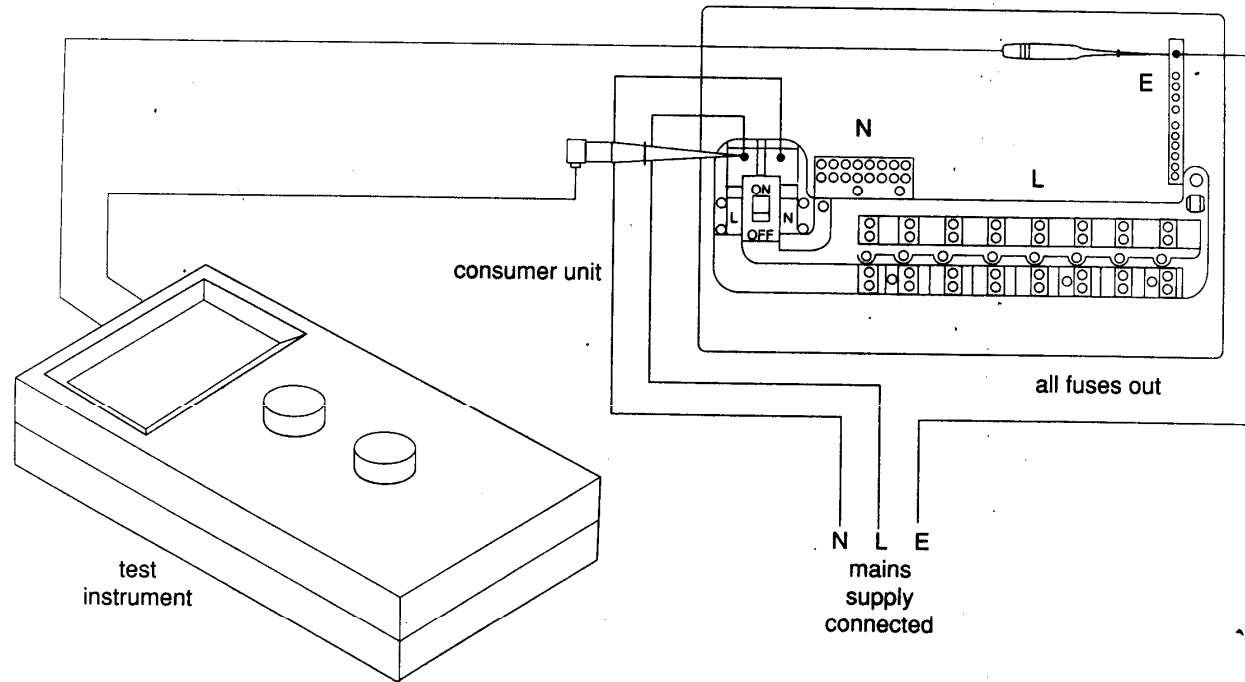
Fig.10.6: Test of Z_0 at the source of supply
