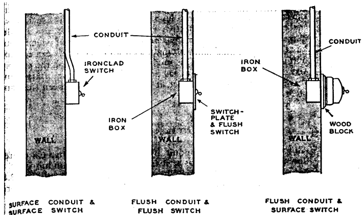
Fig. 5.25. Methods of terminating conduit at switch positions
