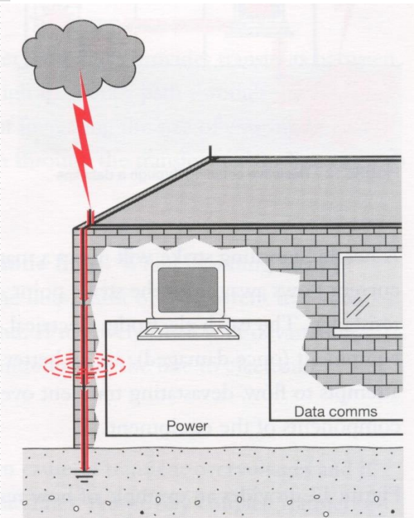
Inductive coupling from a lightning strike on an air rod
