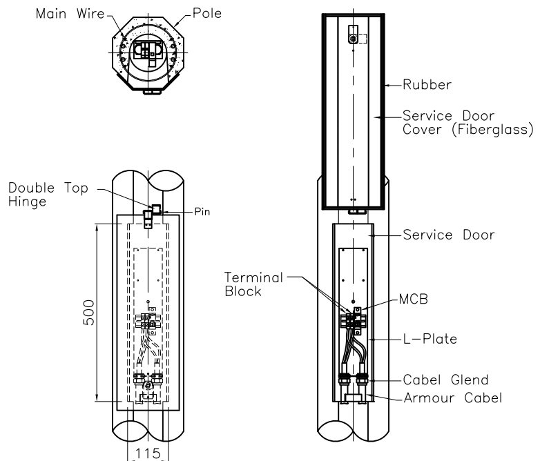
Service Door Detail Scale:1.5/1
