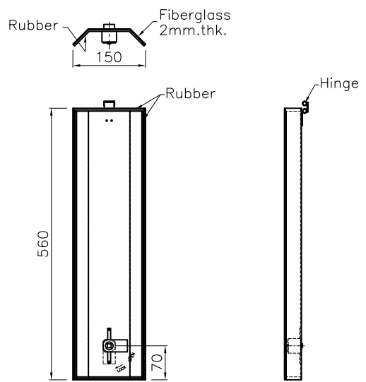
Service Door Cover Scale:1.5/1
