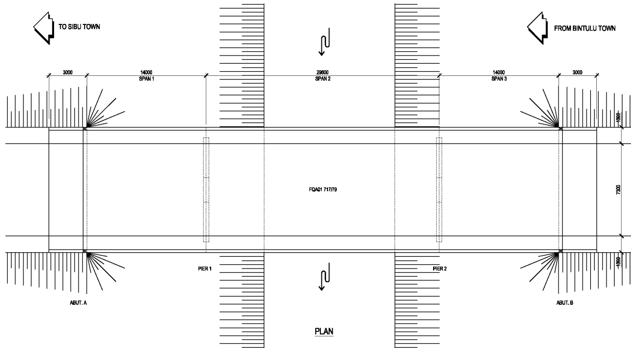
FIGURE 1 GENERAL ARRANGEMENT
