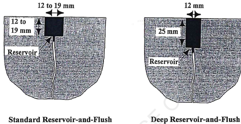
FIGURE 2 – RESERVOIR
