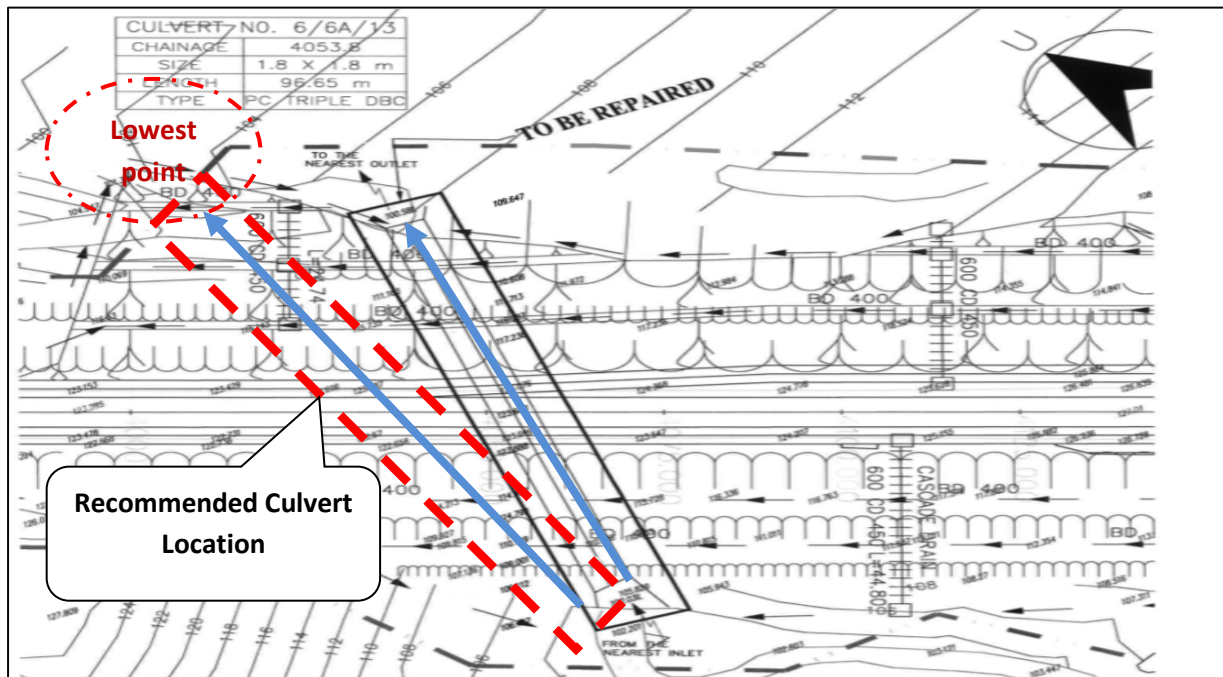
Figure 4.7: Recommended Culvert Location
