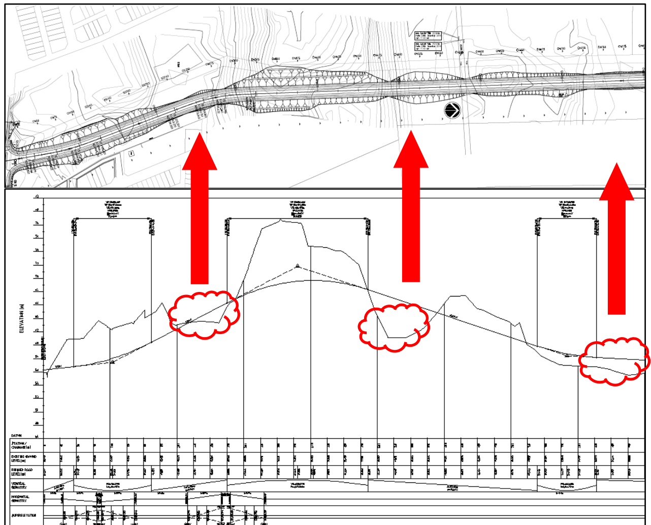
Figure 3.1: Plan and Longitudinal Profile
