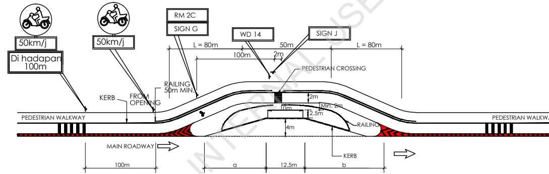
MOTORCYCLE LANE BEHIND BUS STOP (TYPE 1)
