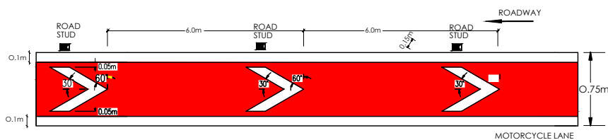
DETAIL A CHEVRON SEPARATOR MARKING FOR NEML ALSO KNOWN AS LINE TYPE 16
