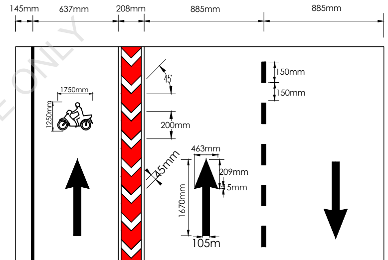
Inset Dimensions
