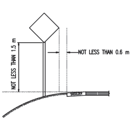
TRAFFIC SIGN (RURAL AREAS) WITH PAVED SHOULDER
