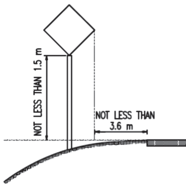
TRAFFIC SIGN (RURAL AREAS) WITHOUT PAVED SHOULDER
