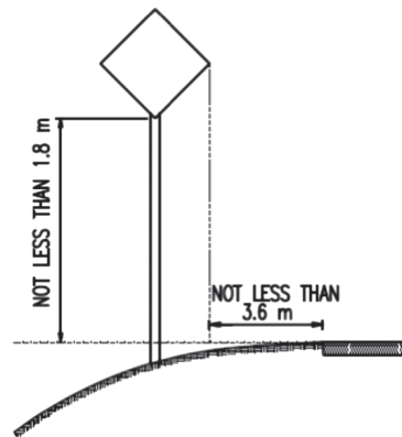
TRAFFIC SIGN (DIVIDED HIGHWAYS) WITHOUT PAVED SHOULDER
