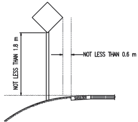
TRAFFIC SIGN (DIVIDED HIGHWAYS) WITH PAVED SHOULDER
