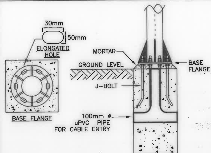
DETAIL 5 : BASE FLANGE & CONCRETE FOUNDATION
