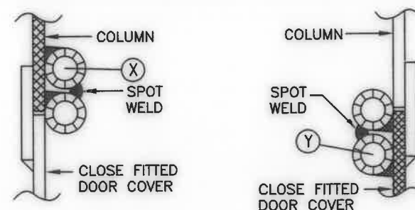
SECT A-A SECT B-B DETAIL 3 : DOUBLE SLOT HINGE
