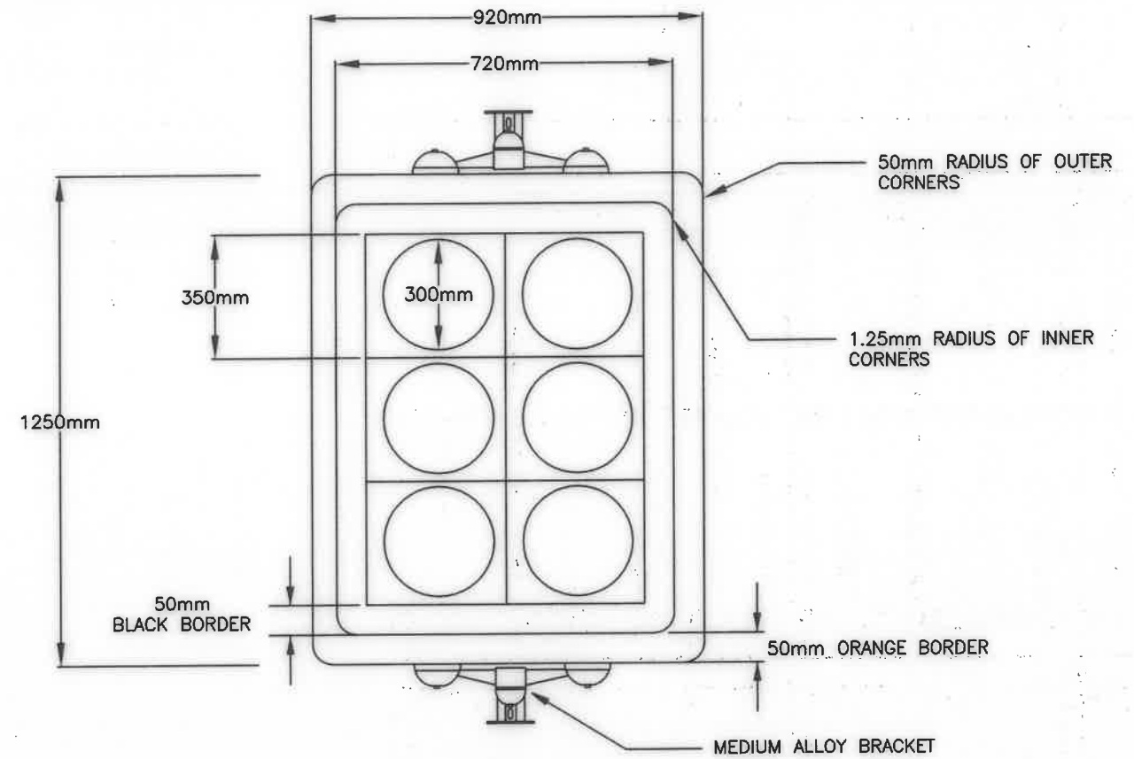
FRONT VIEW (6 X 300 mm TYPE)
