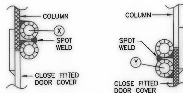
DETAIL 3 : DOUBLE SLOT HINGE
