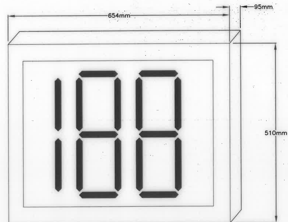
COUNTDOWN NUMERIC DISPLAY (3-THREE DIGIT)
