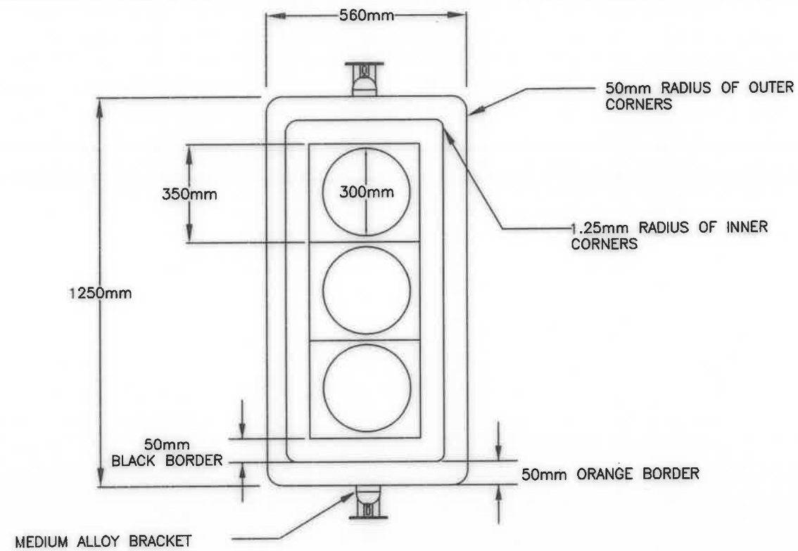
FRONT VIEW (3 X 300mm TYPE)
