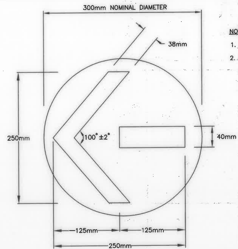
300mm DIRECTIONAL LENS
