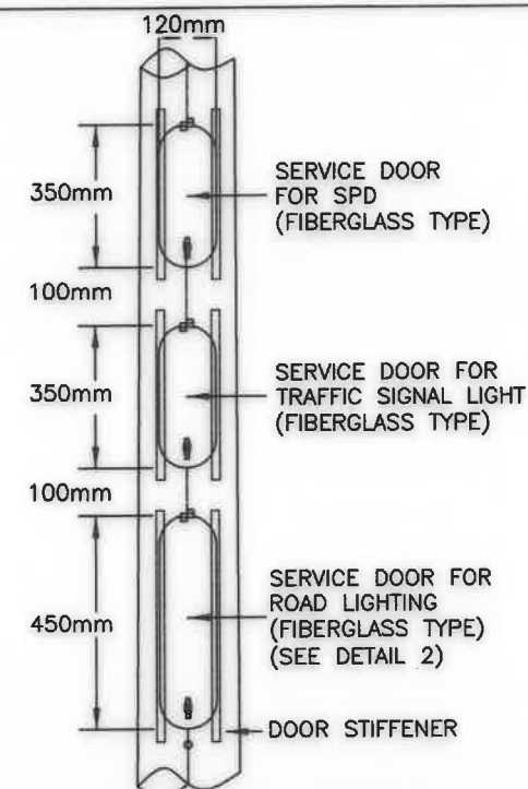
DETAIL 1 : 3 SERVICE DOORS
