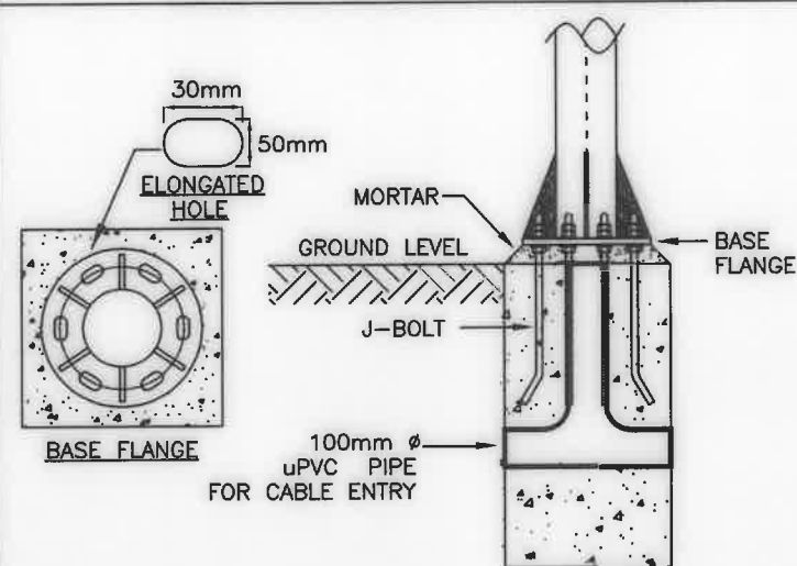
DETAIL 5 : BASE FLANGE & CONCRETE FOUNDATION
