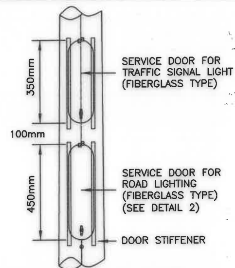
DETAIL 1 : 2 SERVICE DOORS
