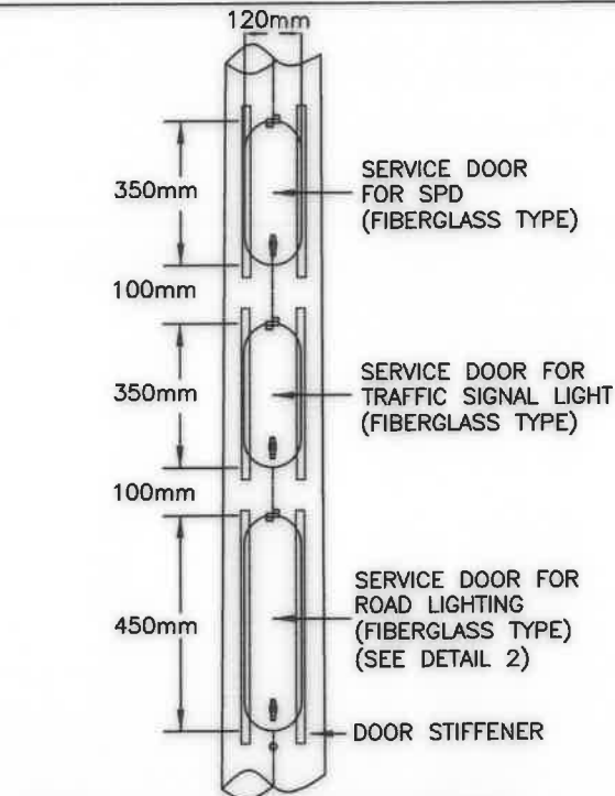
DETAIL 1 : 3 SERVICE DOORS
