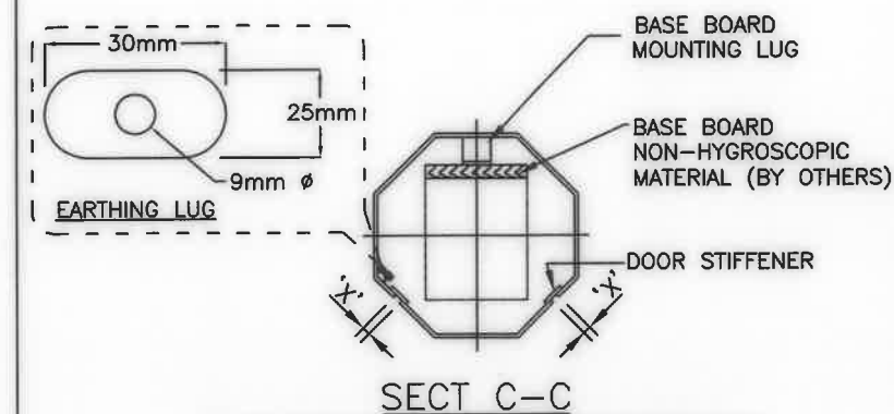
SECT C-C DOOR COVER TO BE MECHANICALLY PUNCH AND THE CLEARANCE - 'X' - AROUND DOOR SHOULD NOT EXCEED 1mm
