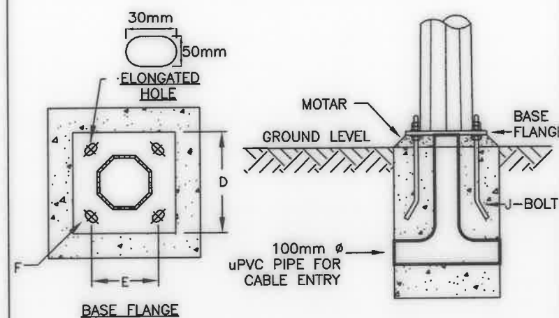
DETAIL 5 : BASE FLANGE & CONCRETE FOUNDATION
