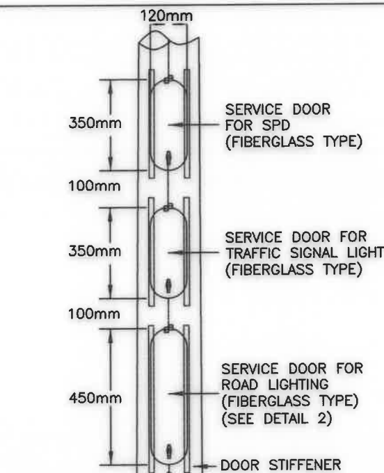
DETAIL 1 : 3 SERVICE DOORS
