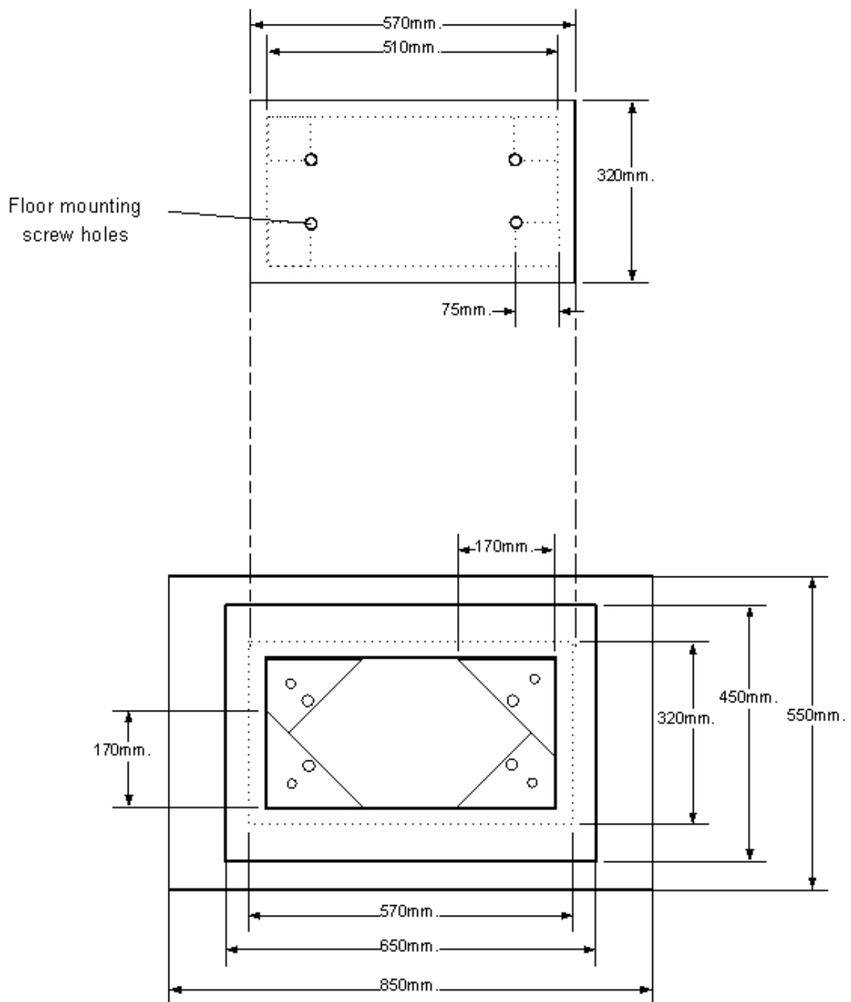
MV/HV, 1 or 2 Feeder Base: Top View
