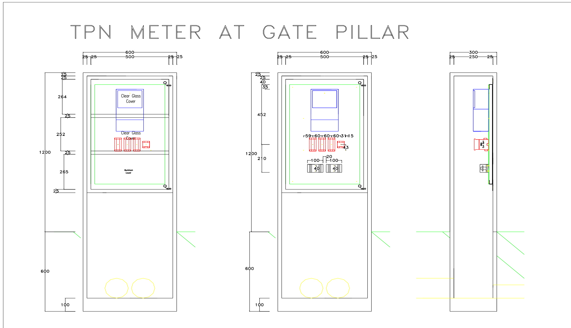
DRAWING NO 1A : METER AT GATE POST
