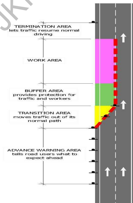
FIGURE 5.2: AREAS IN WORK ZONE
