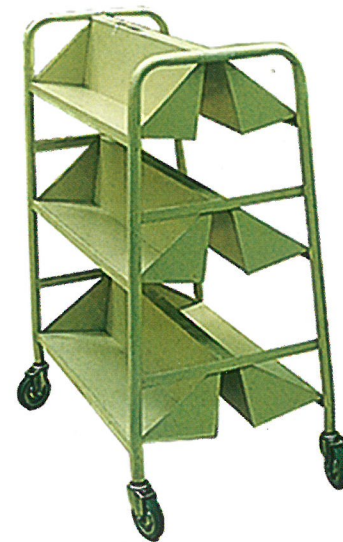
NAGA 045 Book trolley - medium duty Double sided 3 slopping shelves 787W x 508D x 1041H mm
