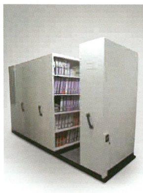
NAGA CC17 MANUAL MOBILE CABINET 1-BAY 6 ROWS Per bay: 1070W x 460D x 2040H mm Overall: 3280mm
