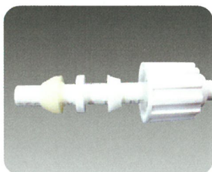
Insert nut compression, clinching ring, spacer & cone into PE-RT Hose (both side)
