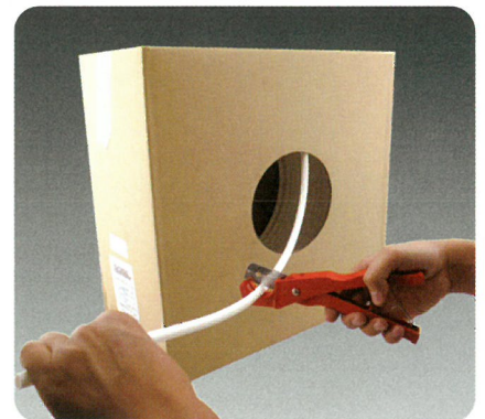
Cut required PE-RT hose length accordingly
