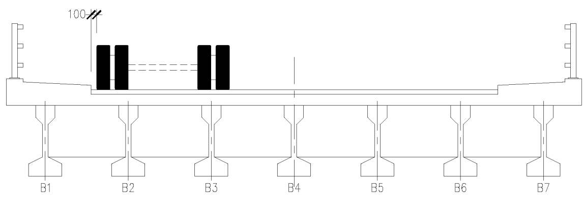
TYPICAL CROSS SECTIONAL
